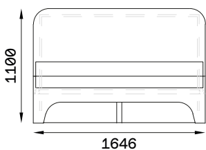
With headboard (flush)
