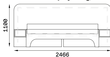
With headboard (projecting)
